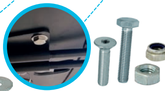
PARAFUSOS (DIN931, DIN933, DIN7991, DIN912), PORCAS (DIN934, DIN985) E ANILHAS (DIN9021, PCL1126, DIN125) Screws, Nuts and Washers / Vis, Nuts et Rondelles / Tornillos, Tuercas y Arandelas
